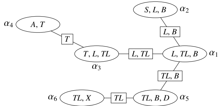
Figure 8.4: Junction tree for the Asia network.
