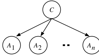
Figure 8.5: Bayesian network representation of a naive Bayes model.
