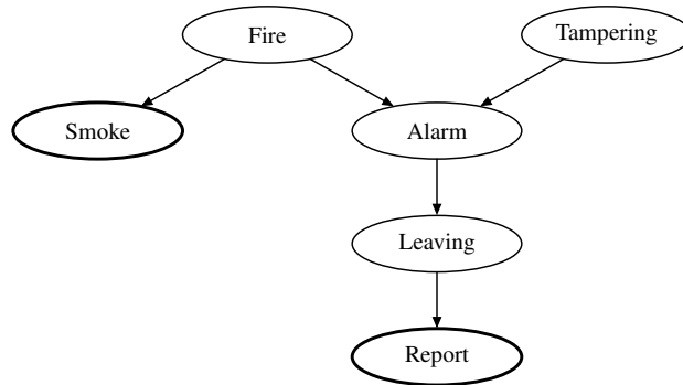
Figure 8.2: Example of a discrete Bayesian network.
