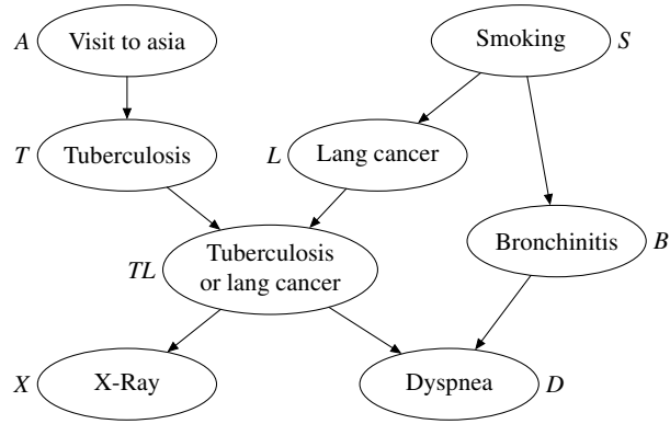
Figure 8.3: Example of a multiply-connected Bayesian network (known as the Asia network).
