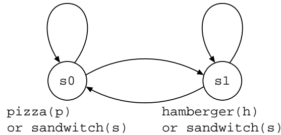
Figure 8.6: State transition diagram of the dieting professor.
